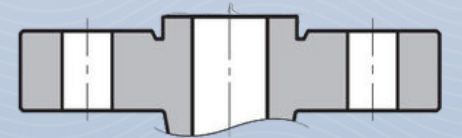
TYPE G AND H - O-RING SPIGOT AND O-RING GROOVE FACE
